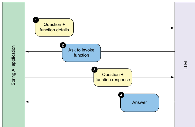
Figure 6.1 Tool invocation involves a multipart conversation between the application and the LLM.
