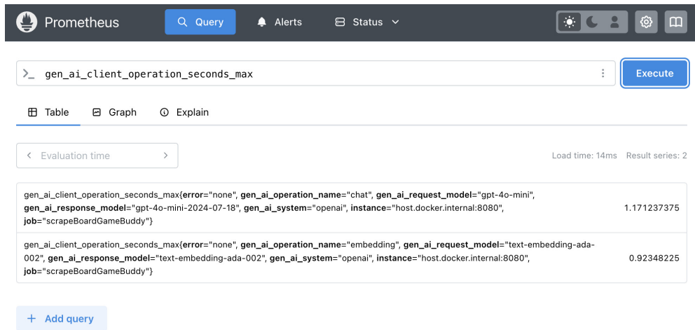
Figure 9.2 Viewing metrics in Prometheus' table view
